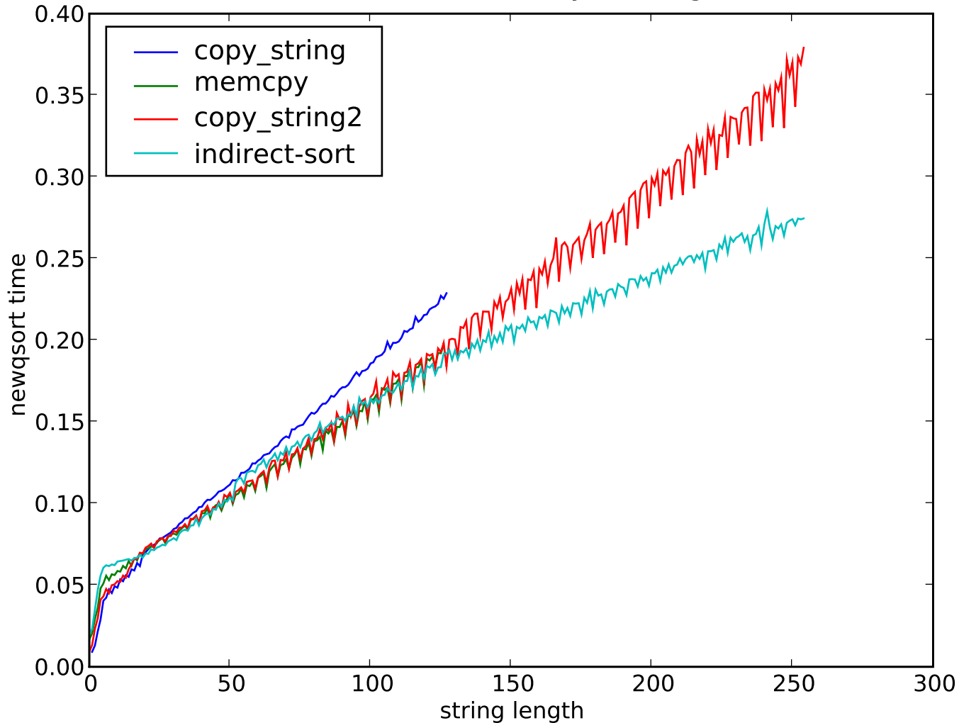
Time to sort an array of strings
